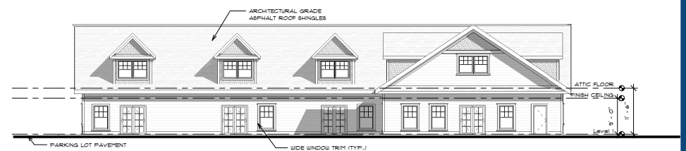
3 REAR ELEVATION 3/32" = 1'-0"
