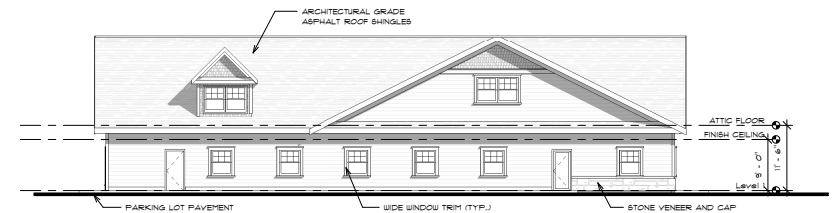
5 LEFT ELEVATION 3/32" = 1'-0"
