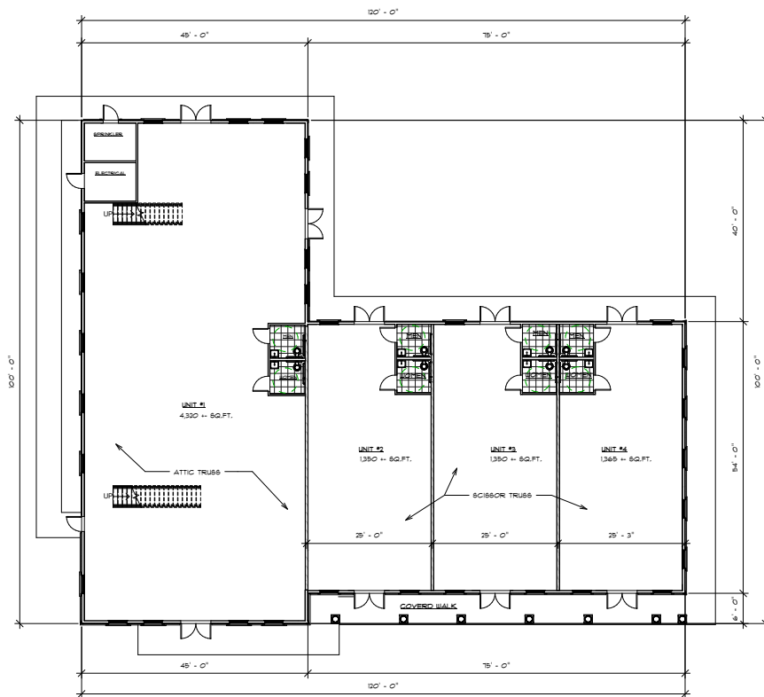
1 Level 1 3/32" = 1'-0"
