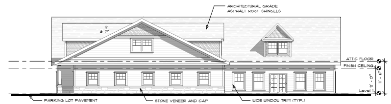
4 RIGHT ELEVATION 3/32" = 1'-0"
