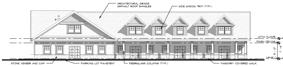
2 FRONT ELEVATION 3/32" = 1'-0"
